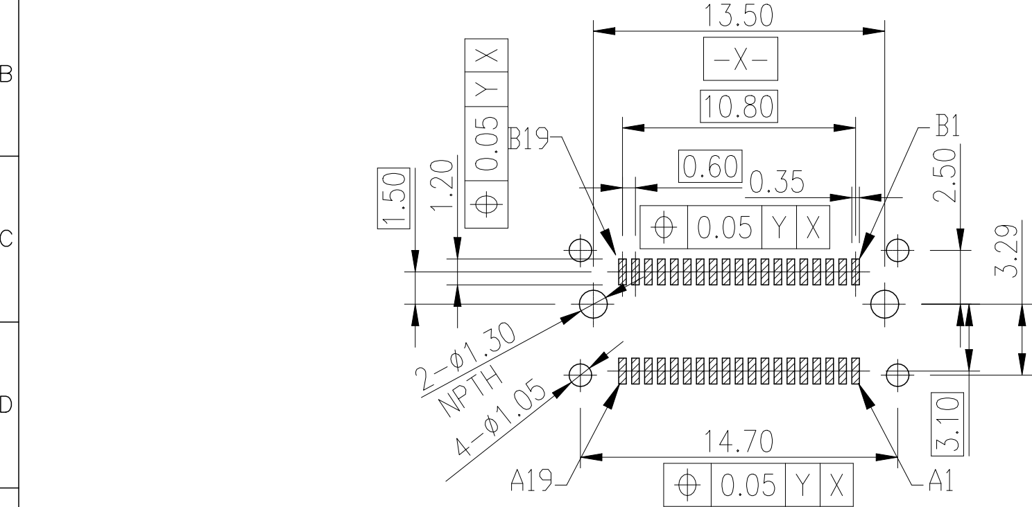
RECOMMENDED PCB LAYOUT GENERAL TOLERANCE: ±0.05
