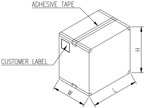
ADHESIVE TAPE
