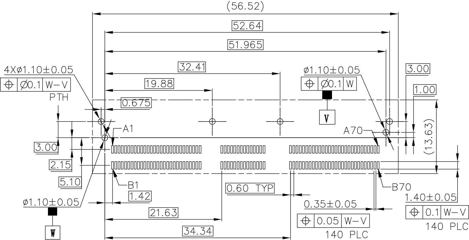
RECOMMENDED 4C FOOTPRINT
