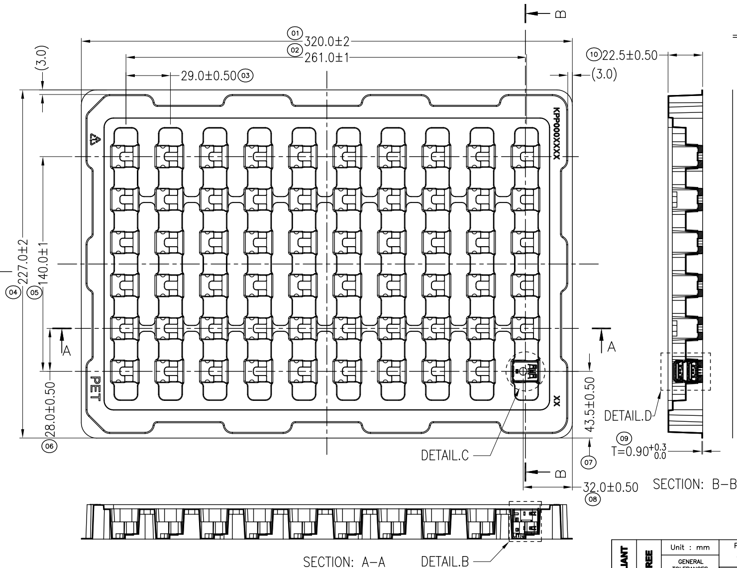
DETAIL.C SCALE 4:1
