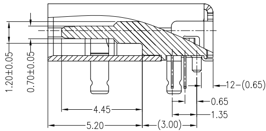
SECTION H-H
